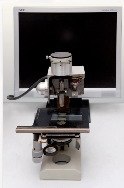
High-frequency acoustic microscope (range 25–100 MHz)
