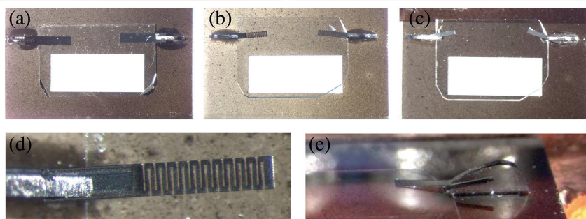
Diamond components for the two-crystal spectrometer module and the beam splitter
