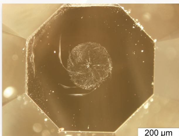
Diamond anvils deformed during synthesis of superhard fullerite: (a) general view of the anvil, (b) \times 3000
